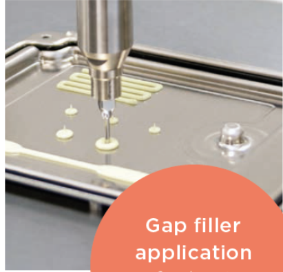
Sealant application to create water tight enclosures
